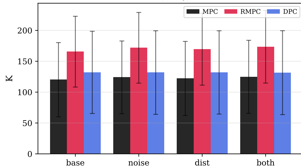
Depth violation rate
