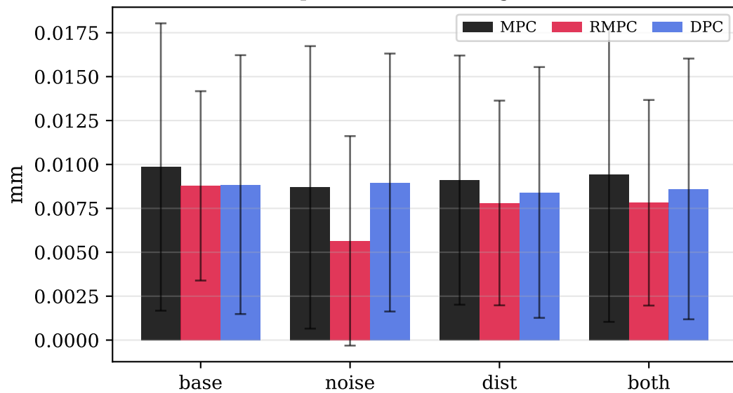
Depth over-bound magnitude
