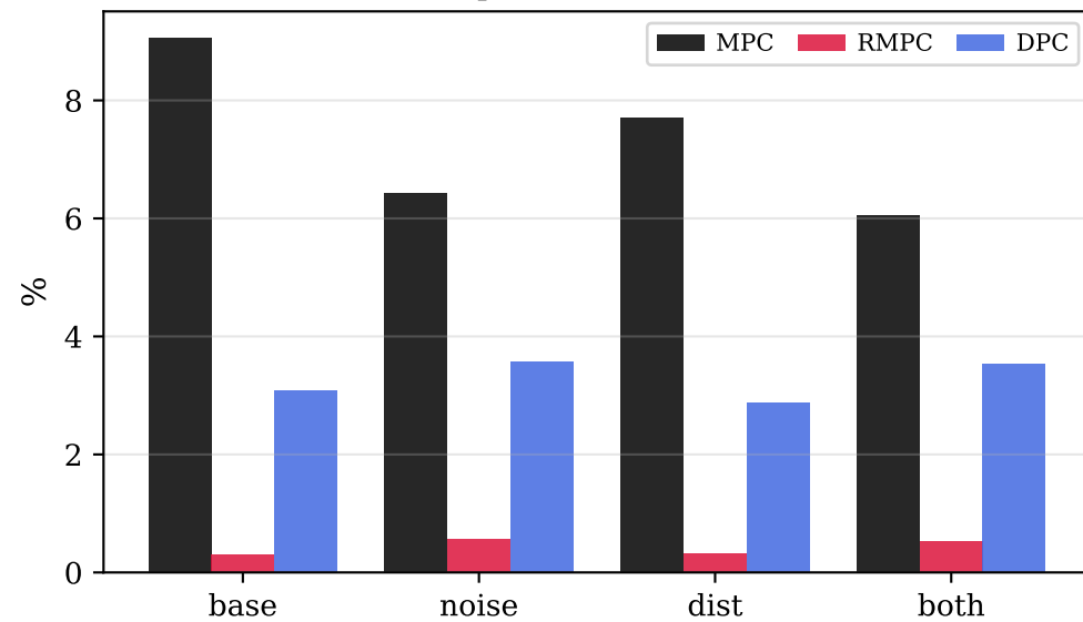
Depth violation rate
