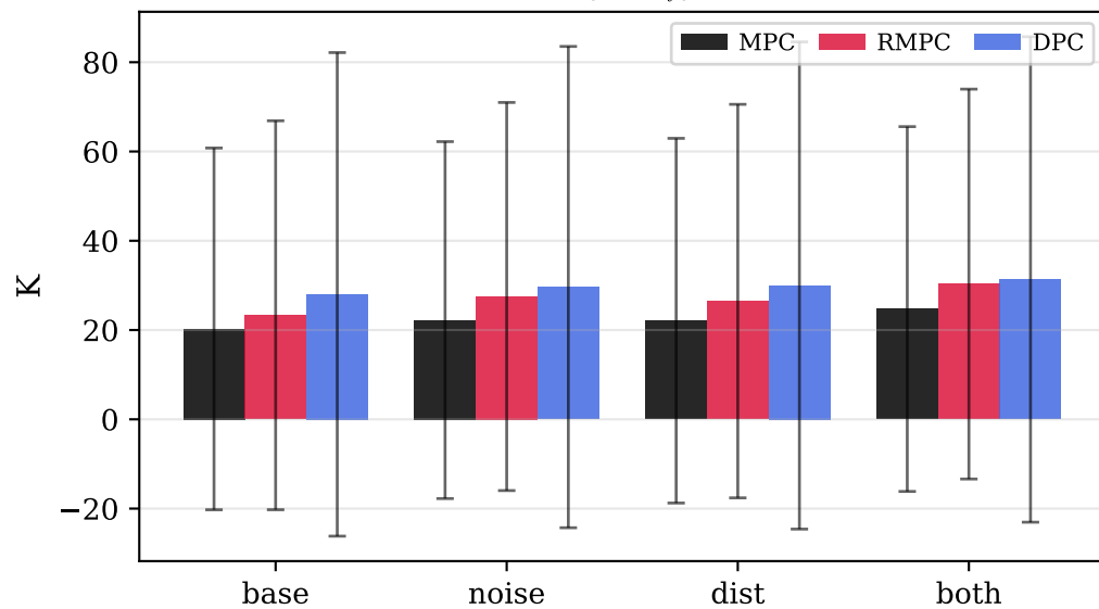
Depth over-bound magnitude
