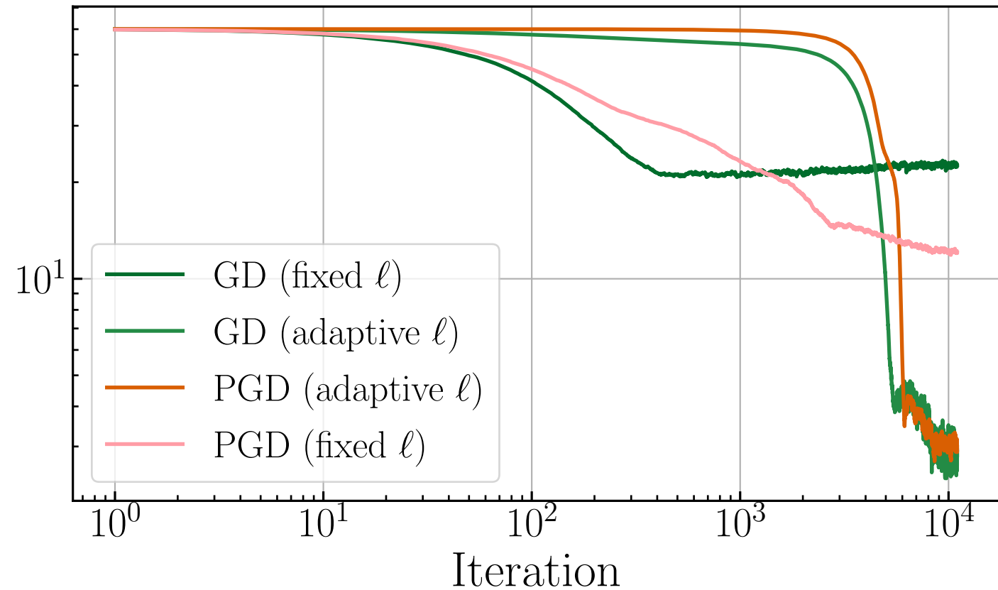
Lotka–Volterra
