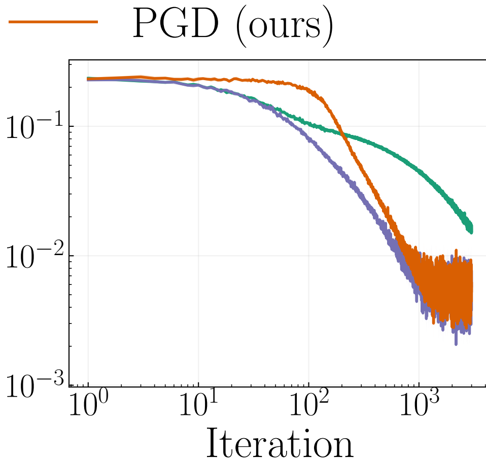
\text{MMD}_{\ell_\infty}(\mathbb{P}_\theta, \mathbb{Q})
