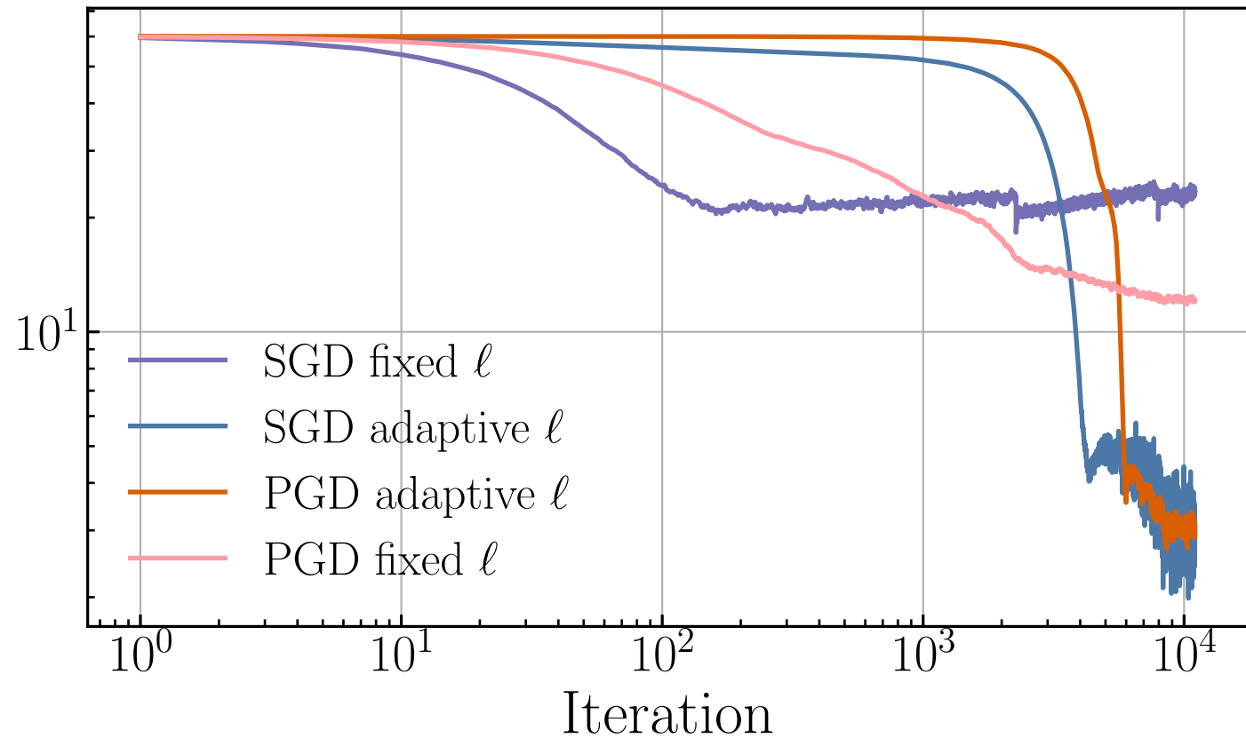
Lotka–Volterra
