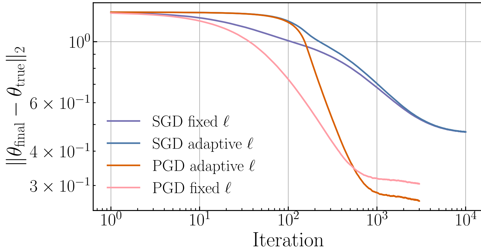
G-and-K
