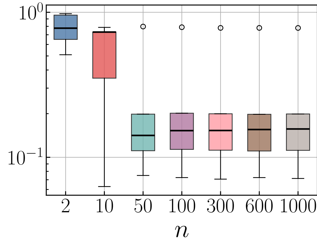
G-and-k distribution
