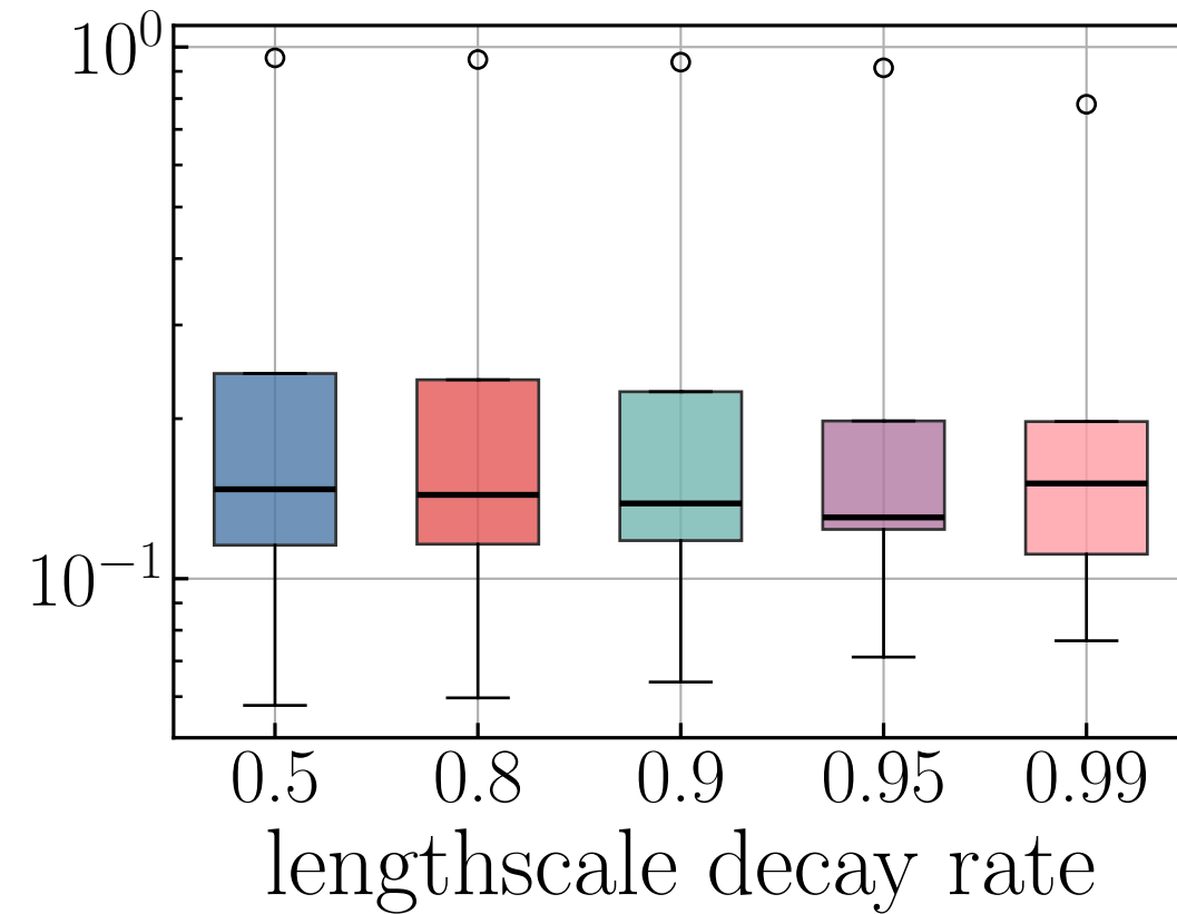
G-and-k distribution
