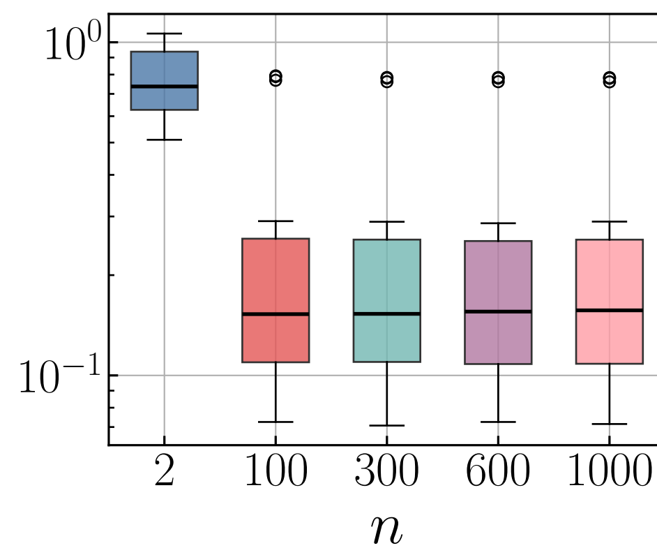
G-and-k distribution
