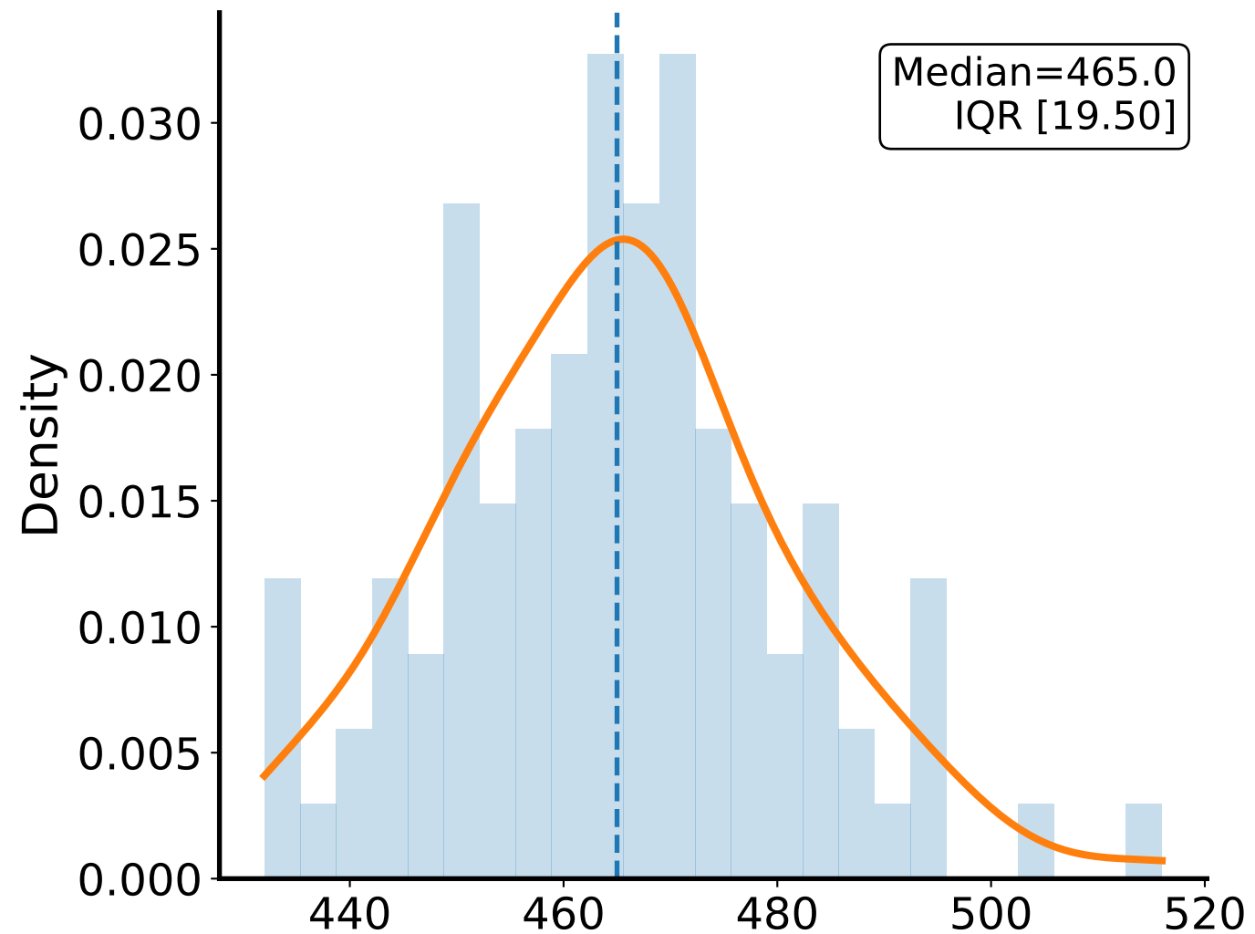
Fixed
