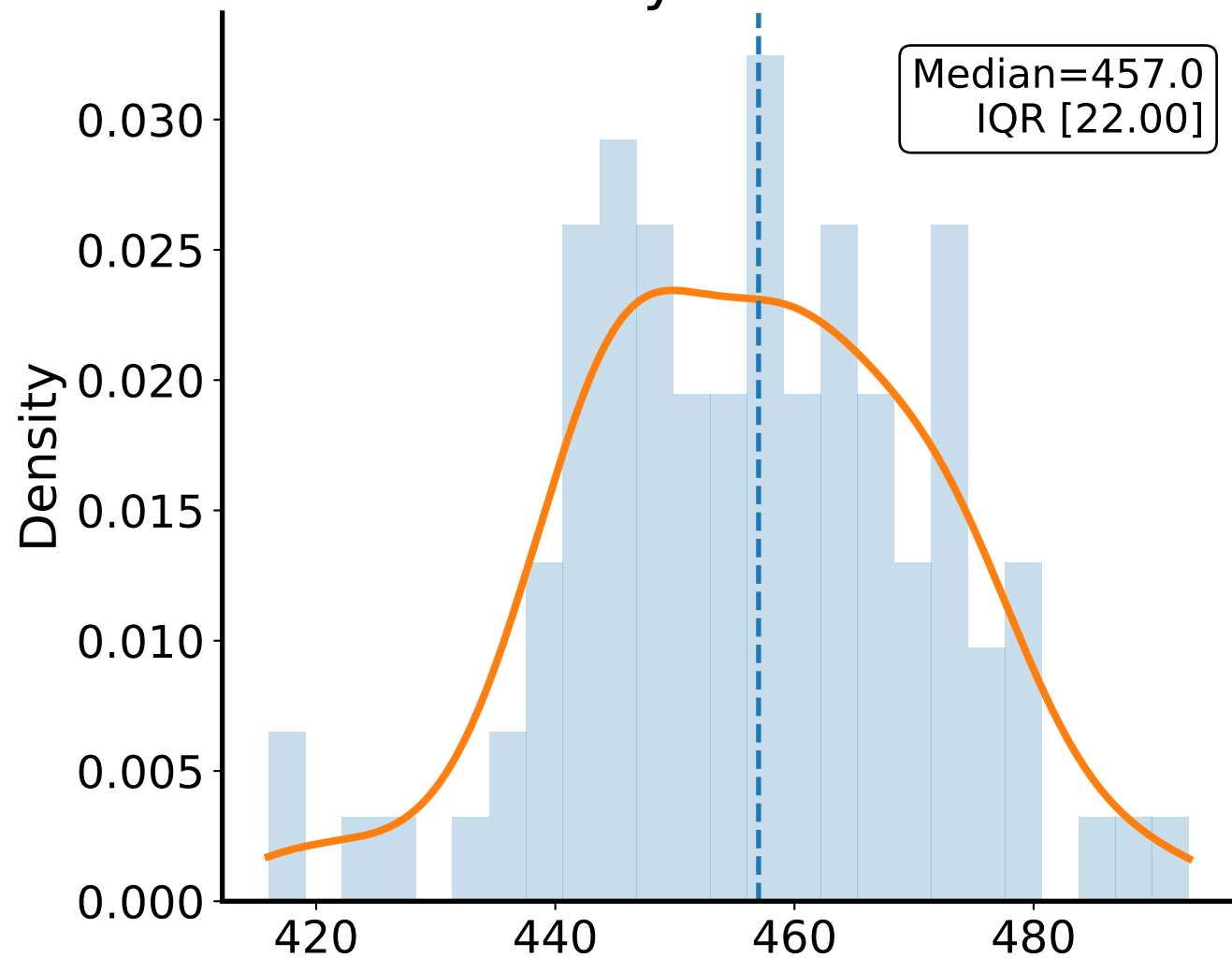
Dynamic
