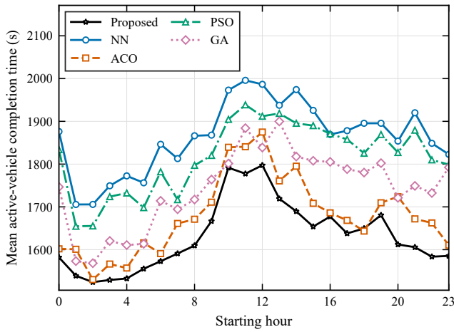
(b) Mean active-vehicle completion time
