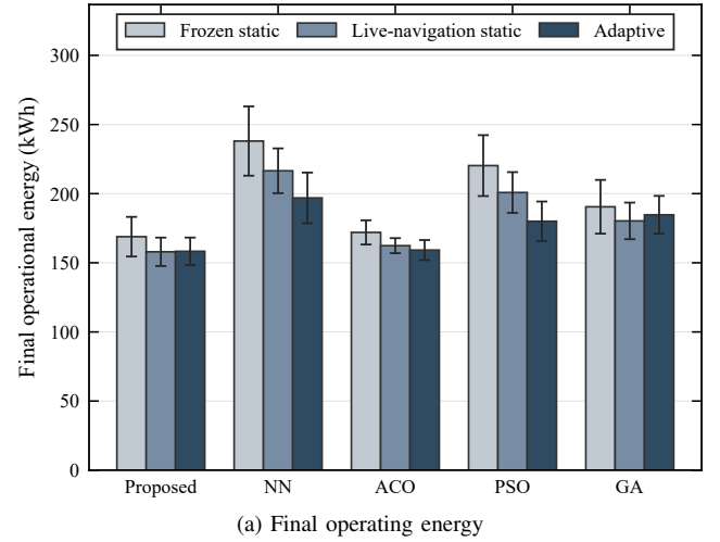
(a) Final operating energy
