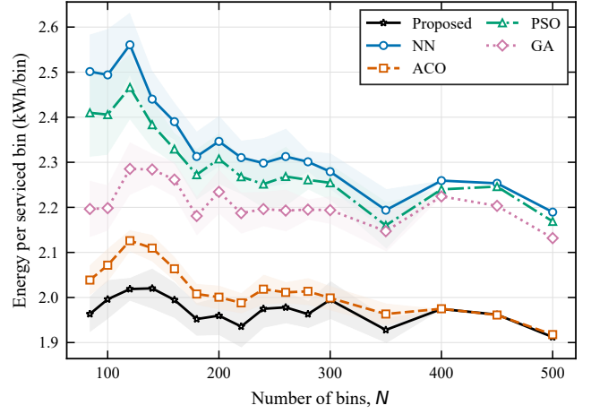
(a) Energy per serviced bin
