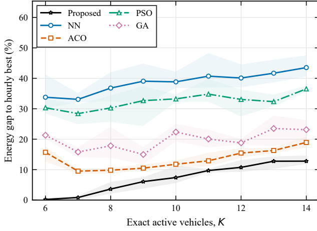
(a) Normalized energy gap
