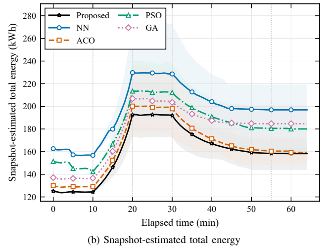
(b) Snapshot-estimated total energy
