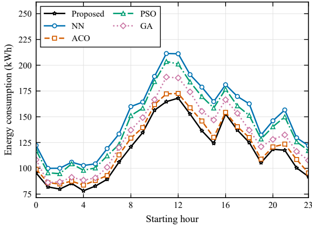
(a) Fleet energy consumption
