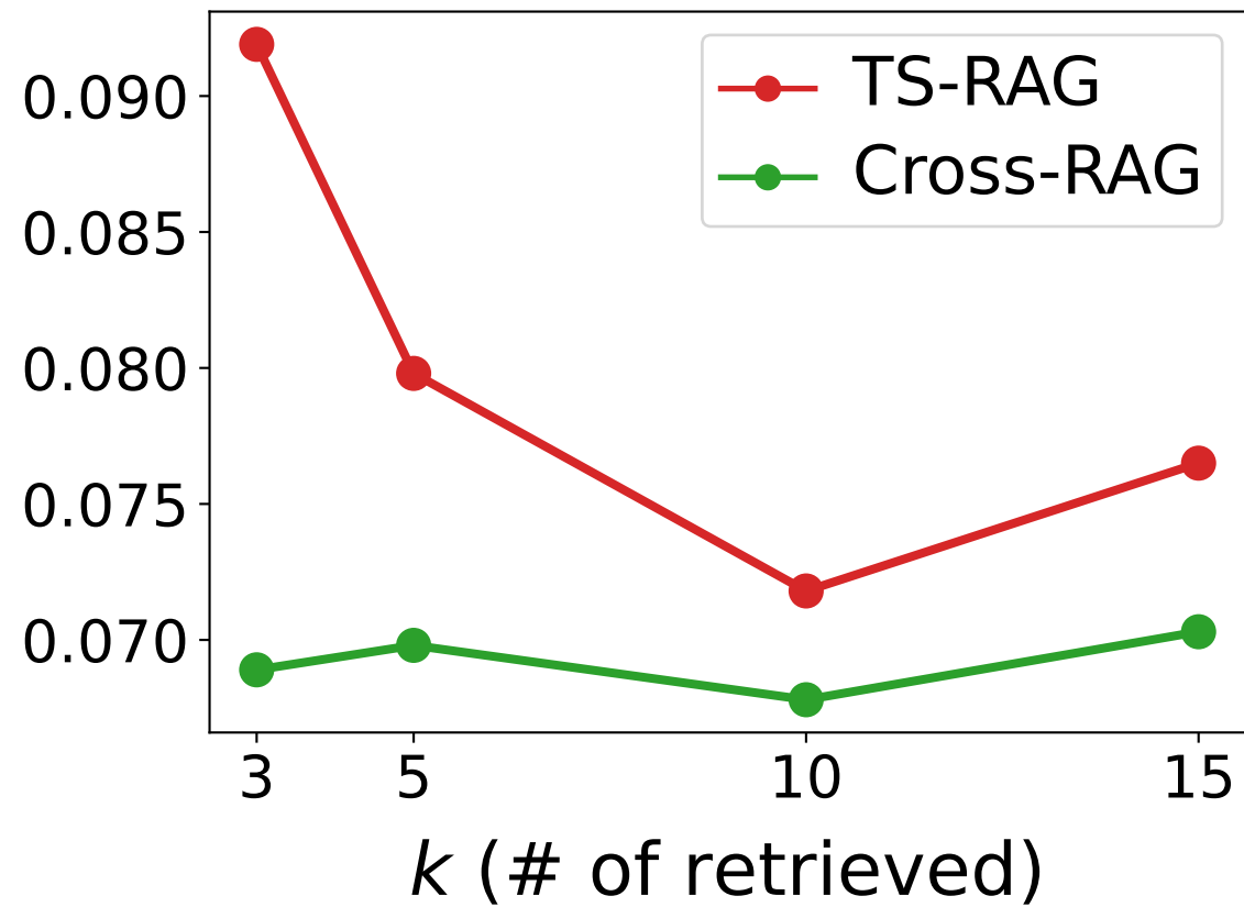
Exchange
