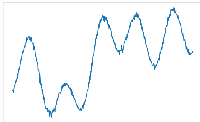
Retrieved: Attention = 0.03
