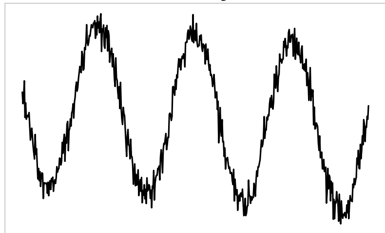
Retrieved: Attention = 0.11
