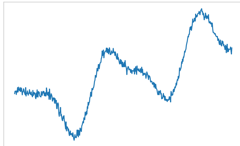
Retrieved: Attention = 0.09
