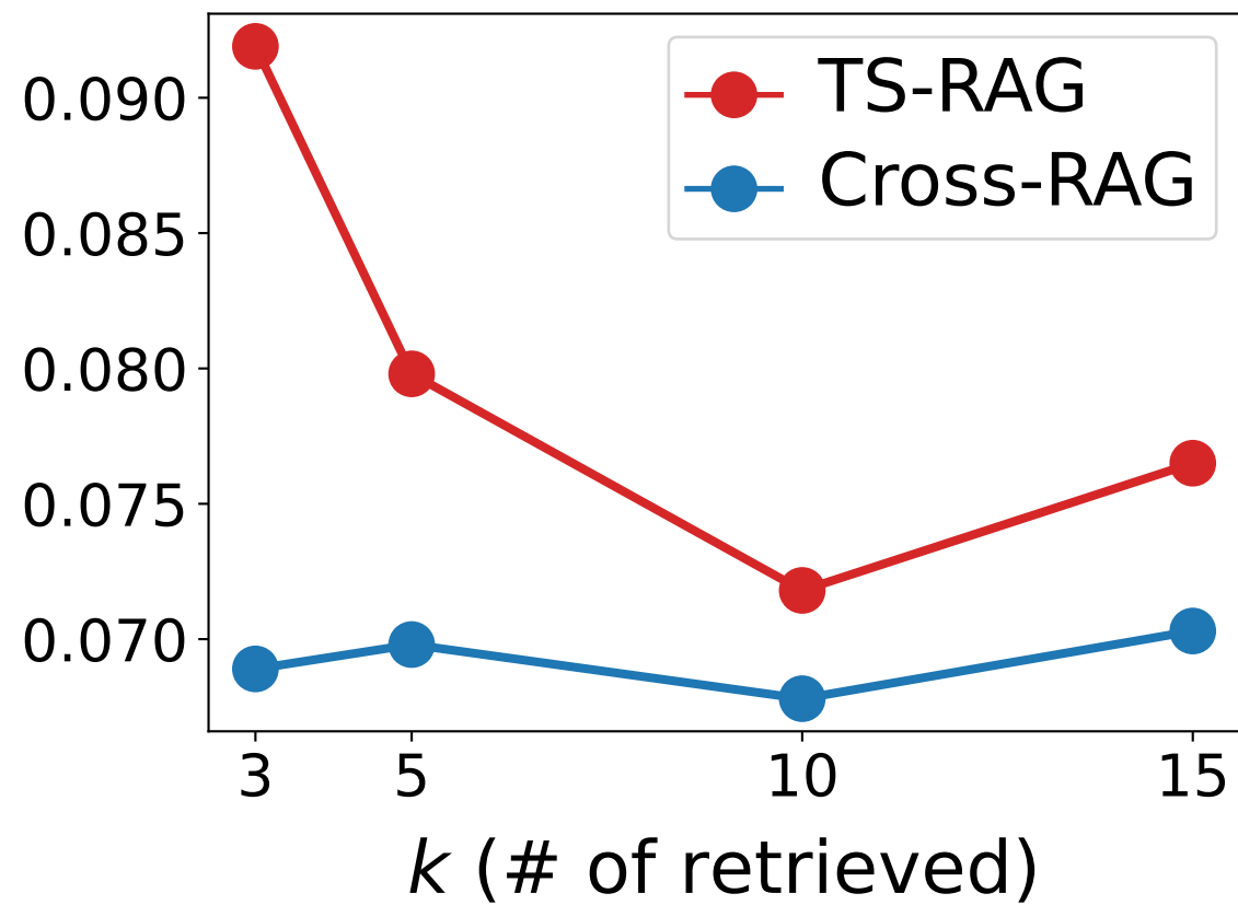
Exchange
