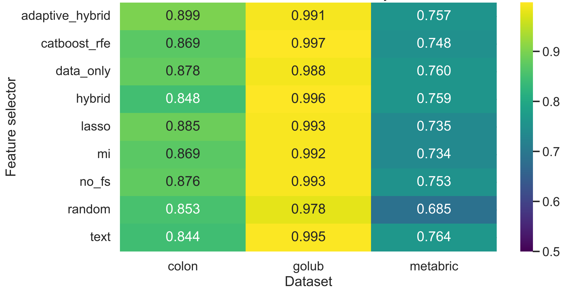
TabPFN AUROC summary
