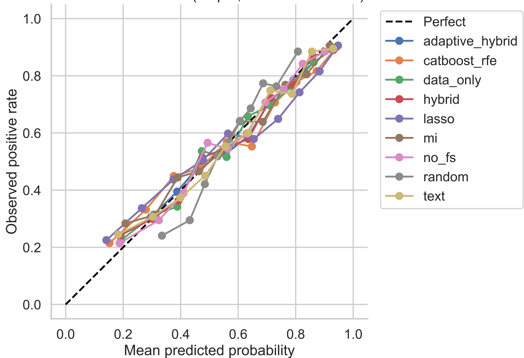
Calibration: metabric (tabPFN, nested-selected k)
