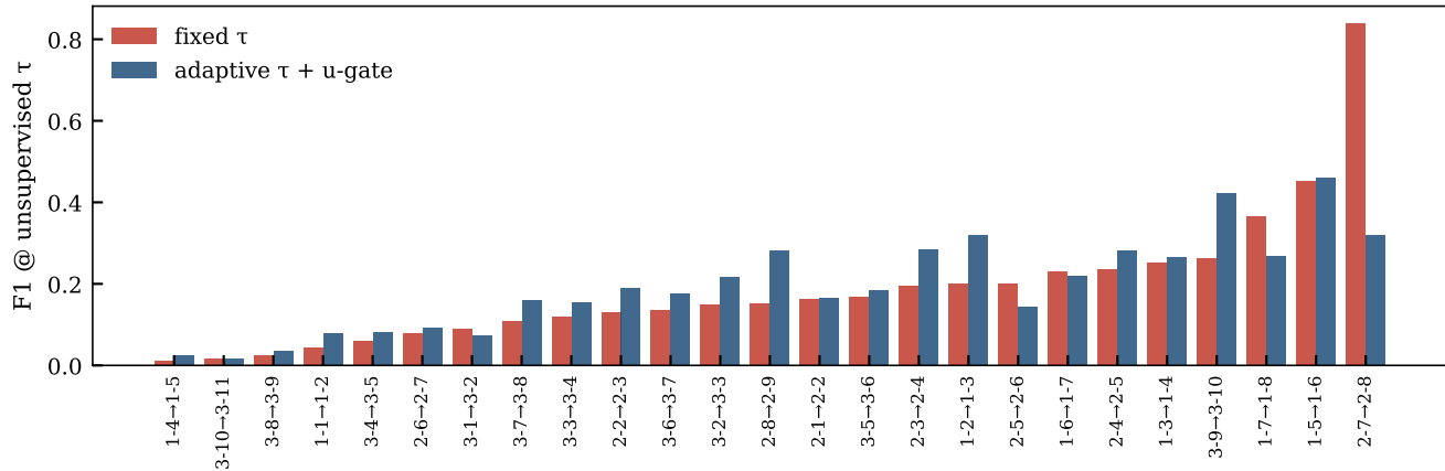
SMD cross-machine shift (train A \rightarrow test B), 25 pairs \times 5 seeds
