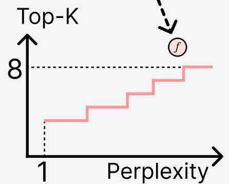
Per-step Policy Piecewise Constant
