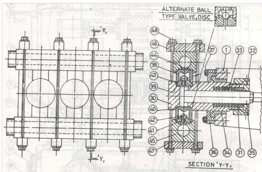
Sectional arrangement, liquid end (alternate ball-type or disc valve shown inset)
