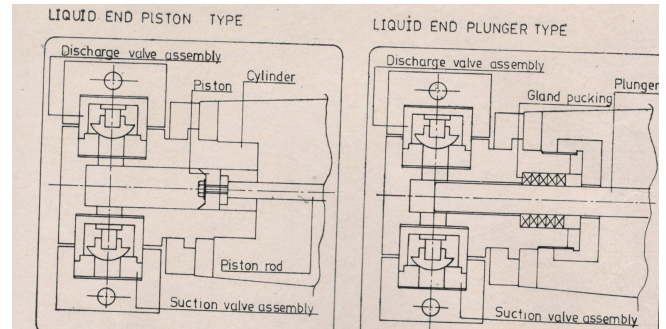
Liquid end: piston type (left) and plunger type (right)
