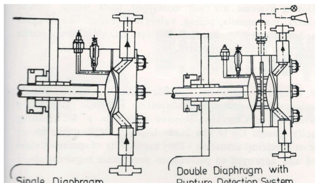
Single diaphragm (left) and double diaphragm with rupture detection (right)
