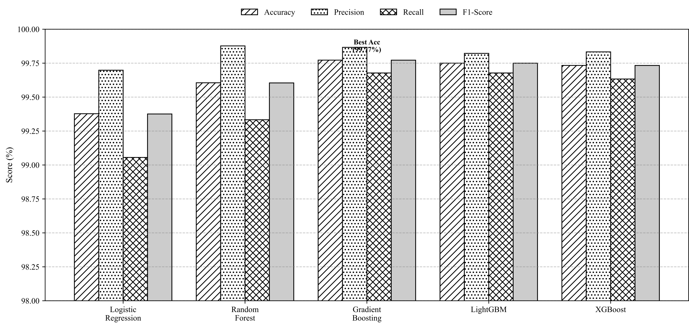
Figure 4. Comparative Performance of ML Models (Real-Time Data)
