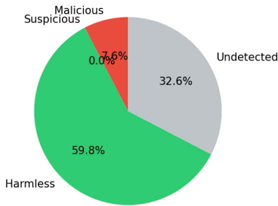
VirusTotal Distribution
