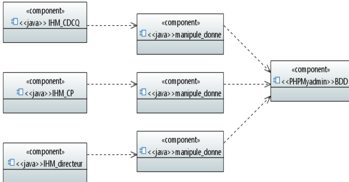
Figure 79 - Diagramme de composant.
