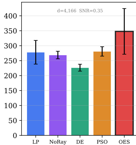
WalkerWalk
