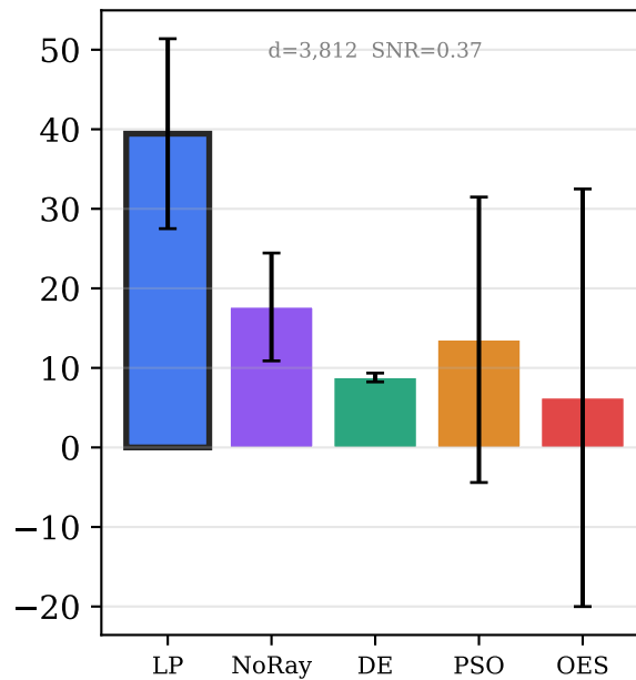
HopperHop
