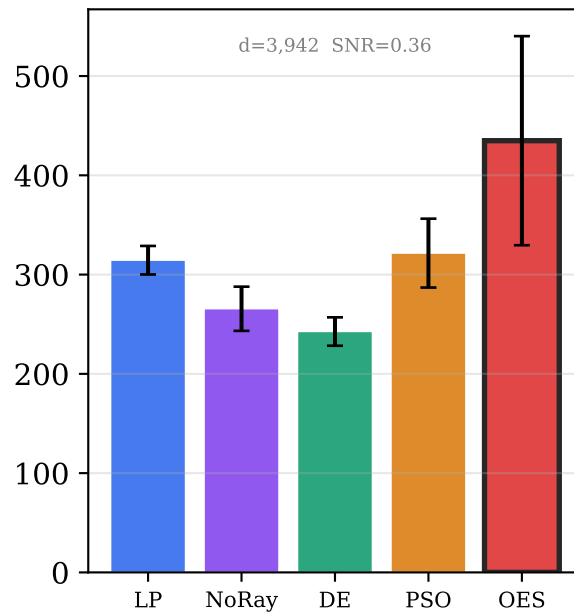
CheetahRun
