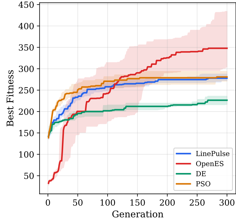
WalkerWalk
