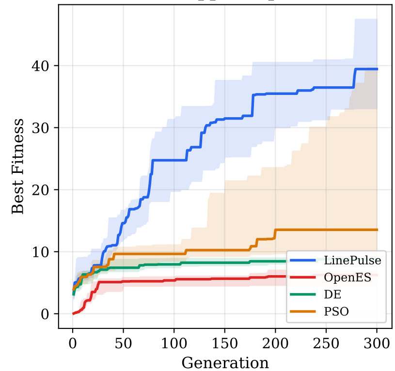
HopperHop
