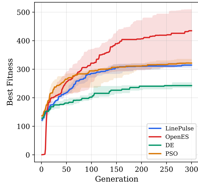
CheetahRun
