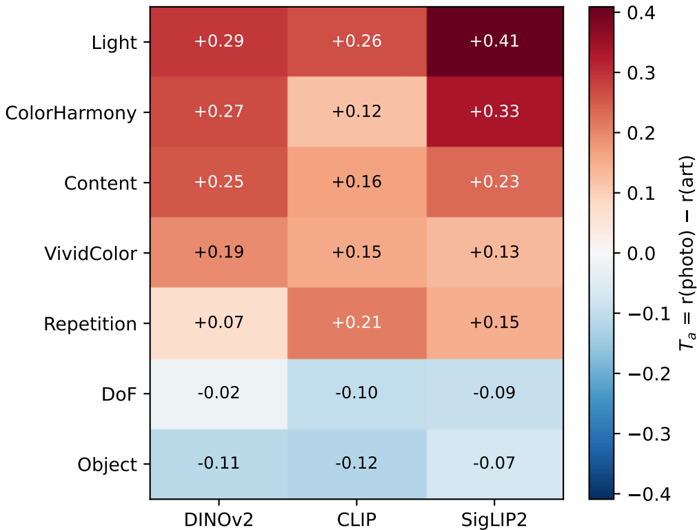
Transfer shift T_a per backbone (Kendall's W=0.849 )
