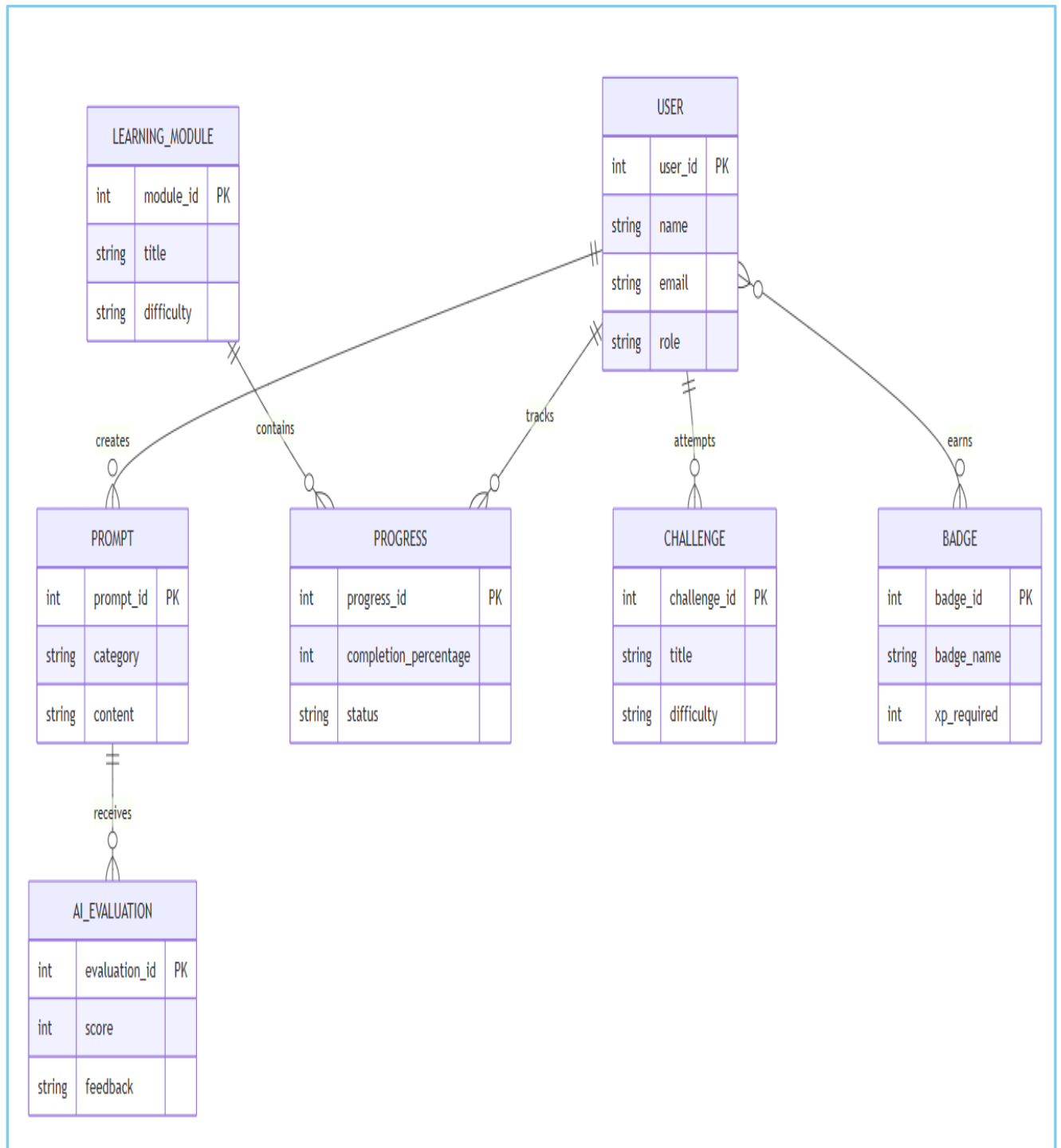
Figure 2: AI Prompt Engineering Learning Hub — ER Diagram
