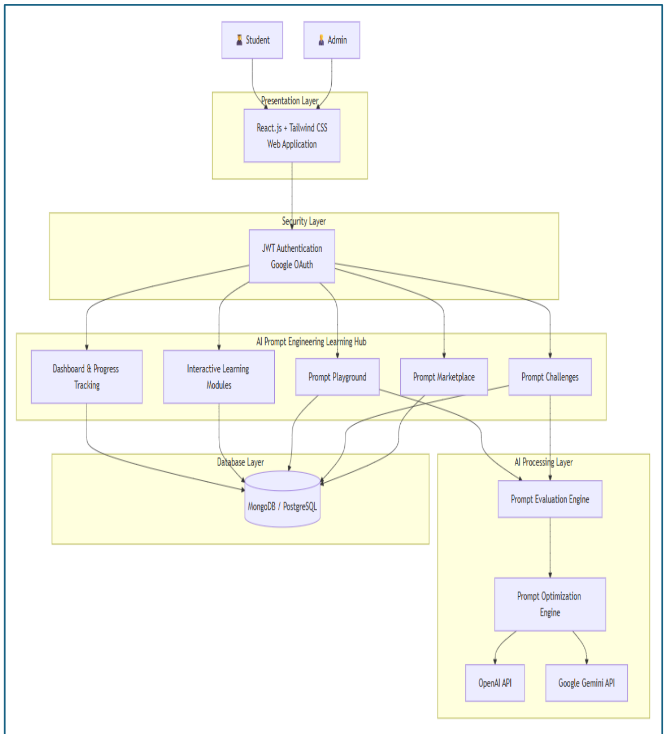
Figure 1: AI Prompt Engineering Learning Hub — System Architecture Diagram
