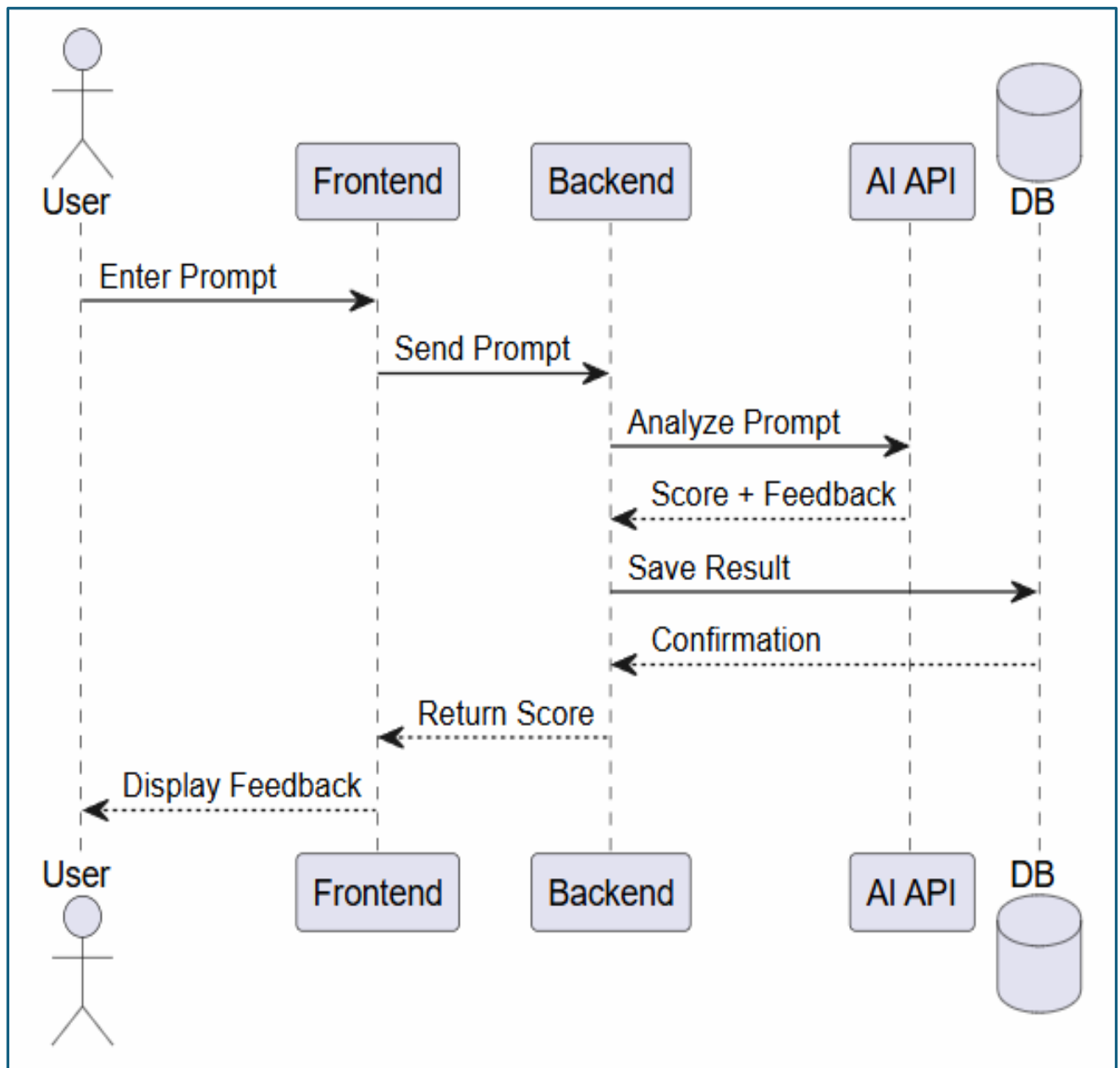
Figure 4: AI Prompt Engineering Learning Hub — Workflow Diagram
