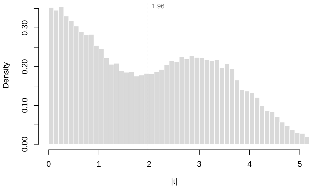
Simulated t-curve
