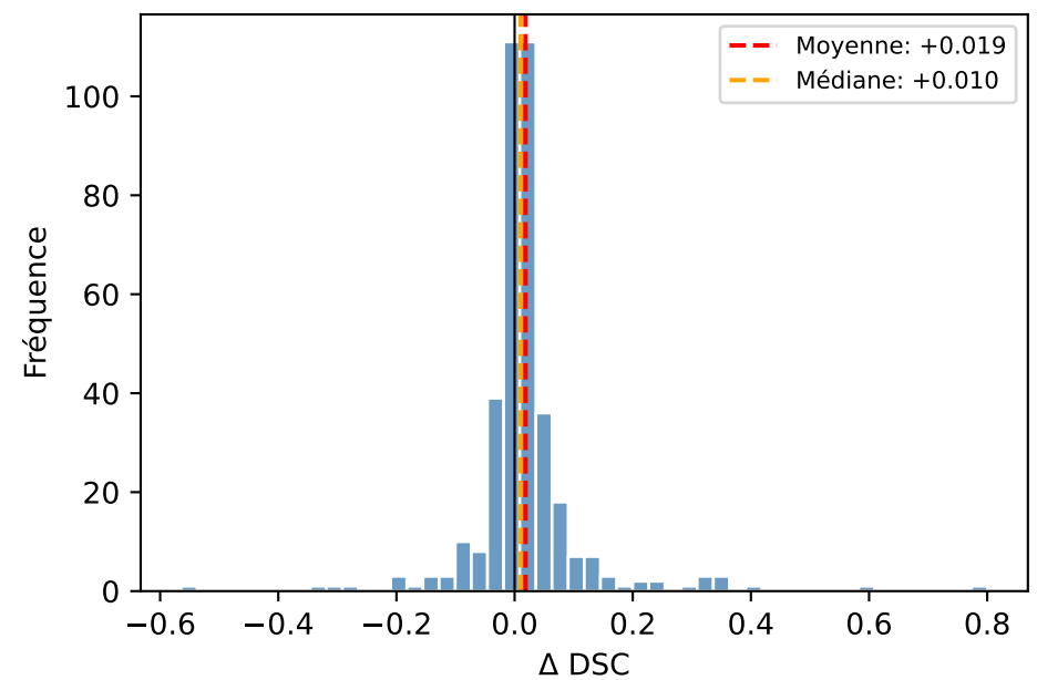
U-Net Final vs U-Net Baseline
