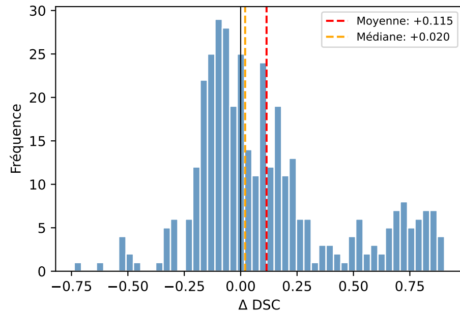
CNN Patch vs K-means LAB
