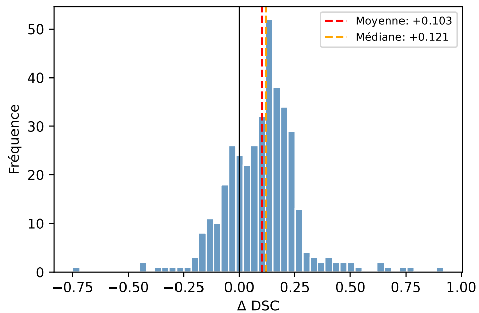
U-Net Baseline vs CNN Patch
