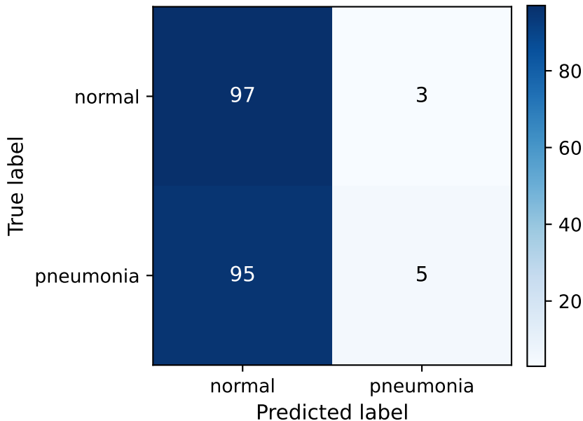
Confusion matrix (LoRA)
