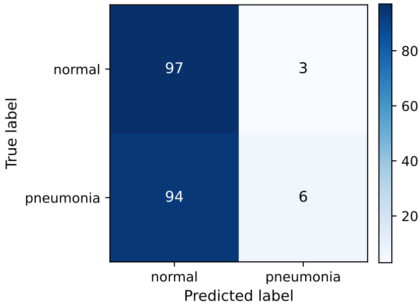
Confusion matrix (zero-shot)
