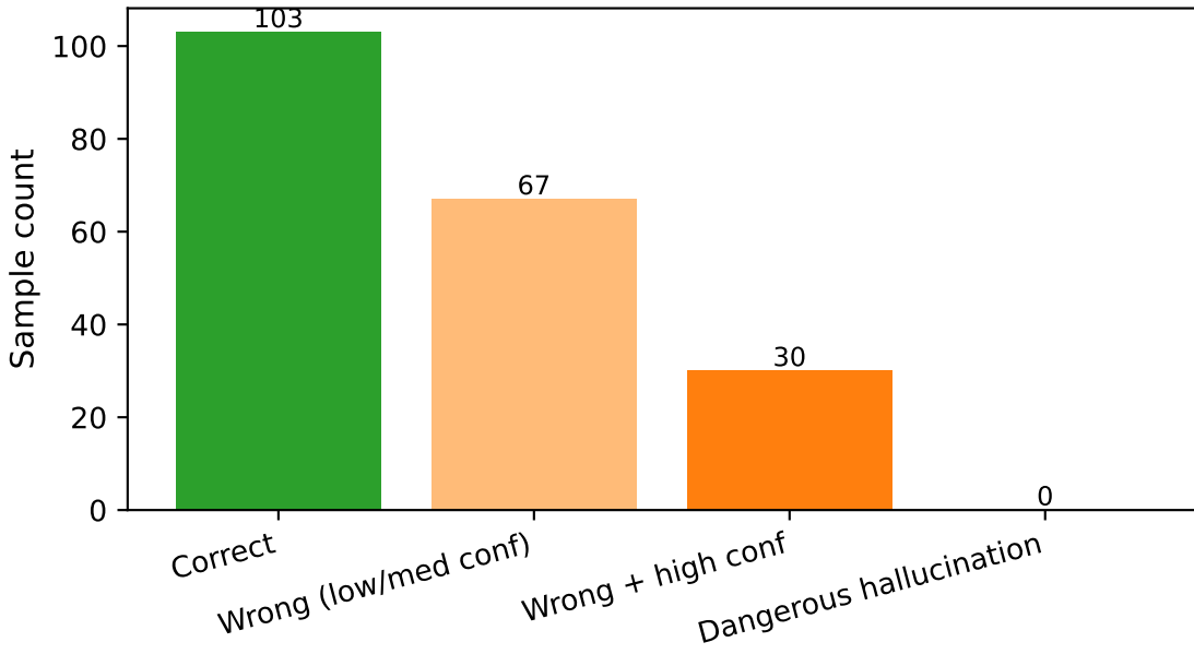
Hallucination breakdown (zero-shot)
