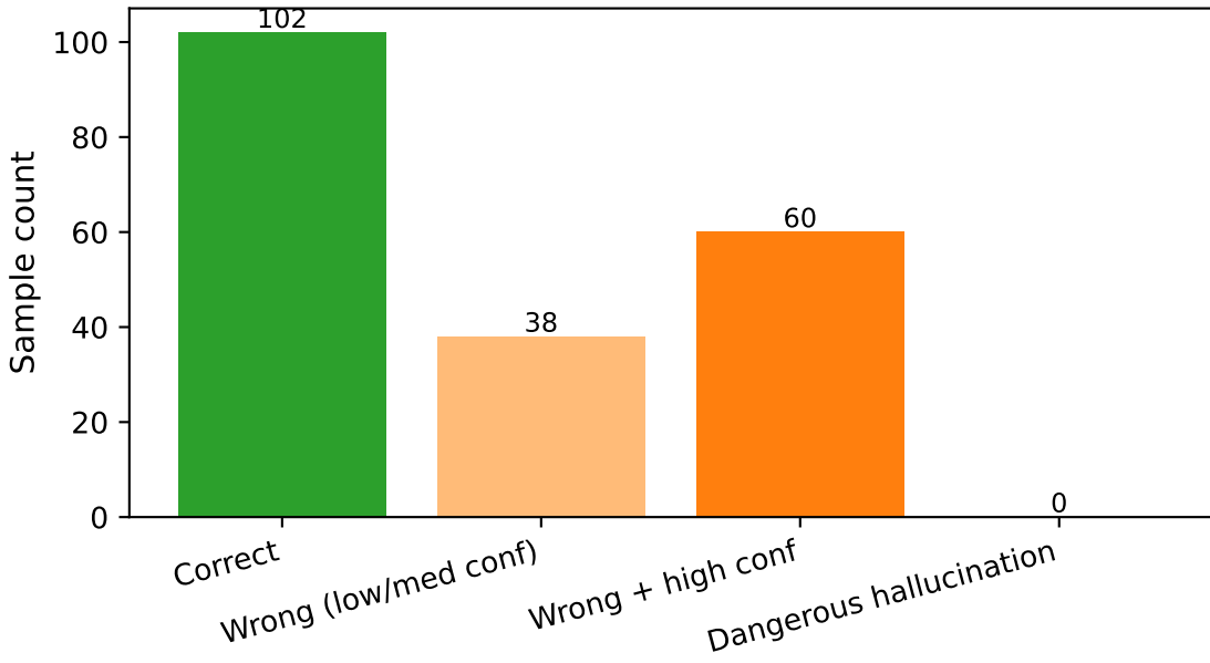
Hallucination breakdown (LoRA)
