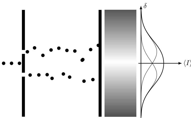
Figure 6.10 Naive expectation of the observed pattern for a double-slit experiment with single photons. This pattern is not observed in a real experiment.
