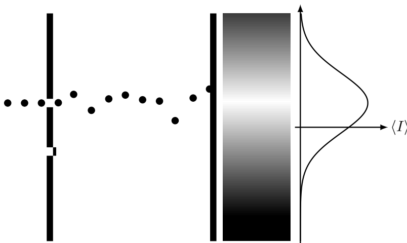
Figure 6.9 Single-slit experiment with single photons.
