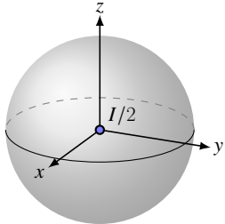
Maximally mixed state
