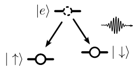
Figure 13.8 Our second idea for a memory qubit is to use the ground-state spin of an atom. This allows us to use a polarized photon as a flying qubit robust against loss.
