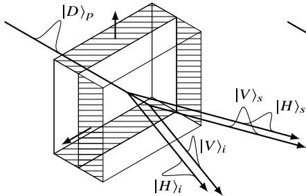
Product photon pair
