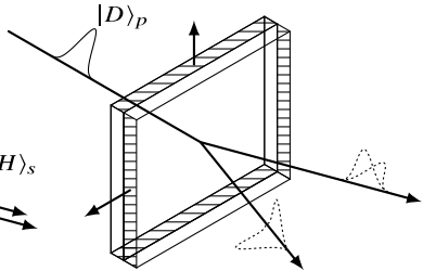
Entangled photon pair
