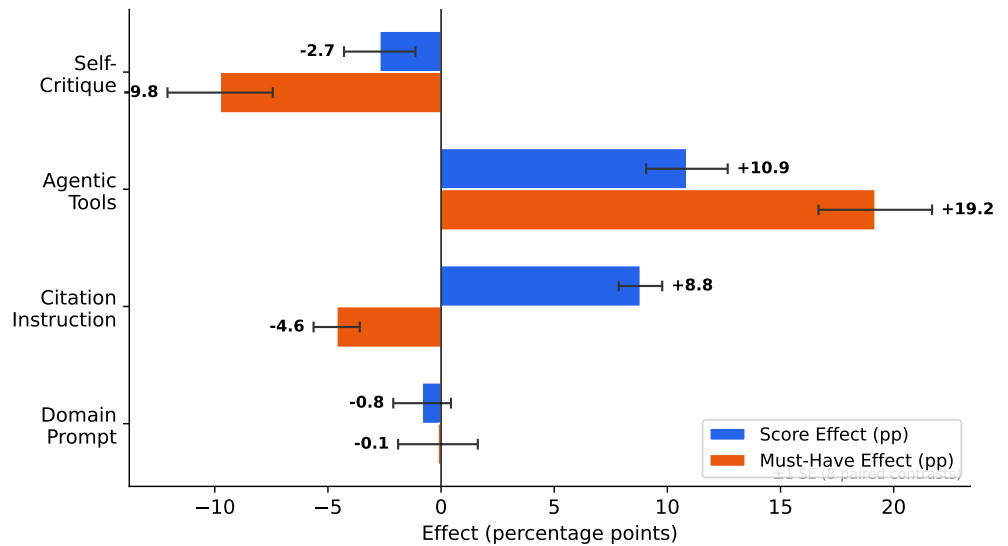
Figure 1. Plot of the average score effect and must-have effect of each augmentation factor, computed across all 8 paired comparisons in the 128-question benchmark. Agentic tools are the only factor that improves both metrics simultaneously; Self-Critique and Domain Prompt are net negative on both.
