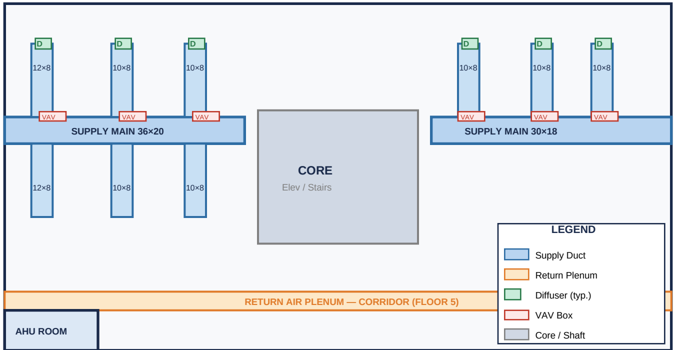
Figure 2 — Typical Floor Duct Layout, Floor 5 (Schematic — Not to Scale)
