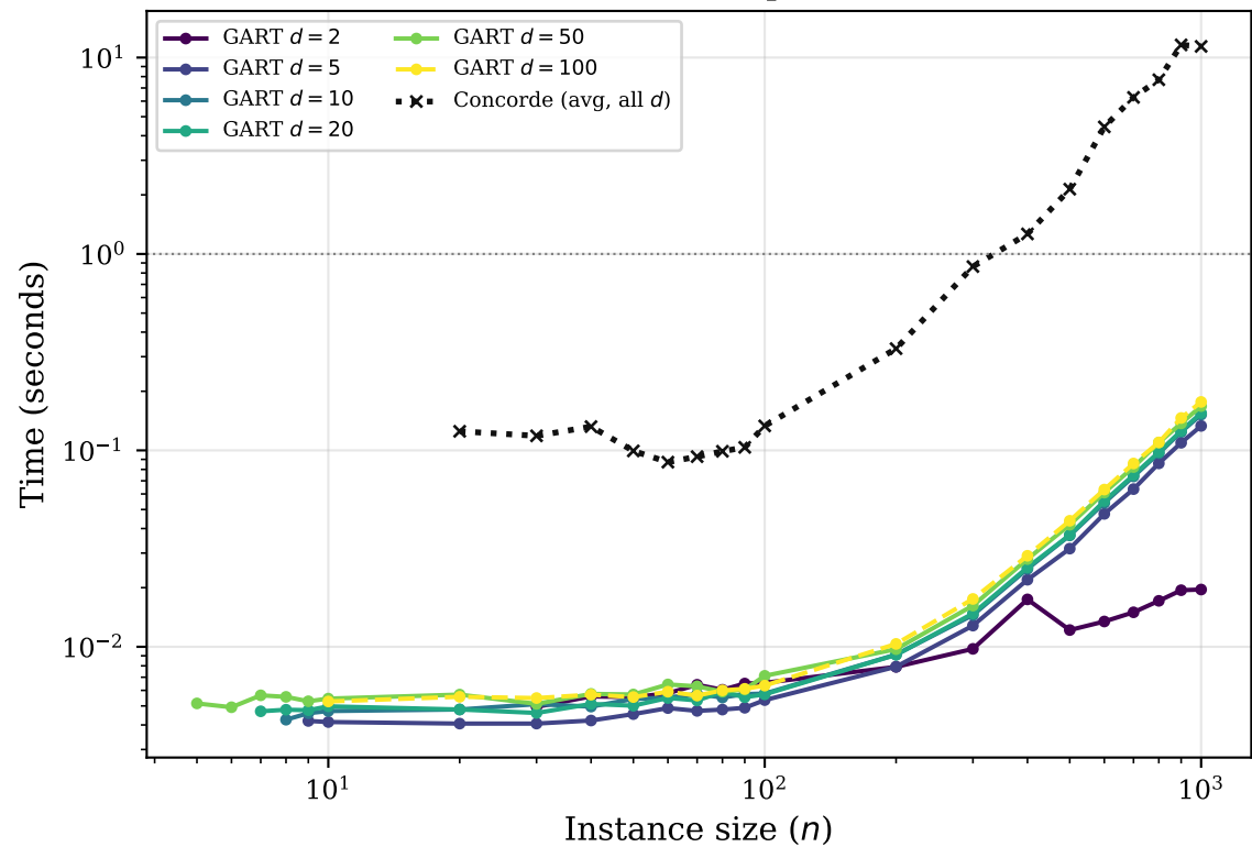
(b) GART vs Concorde prediction time
