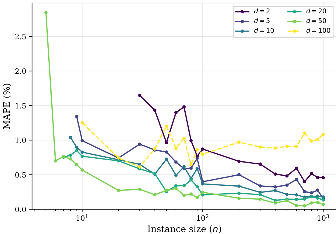
(a) Accuracy across dimensions
