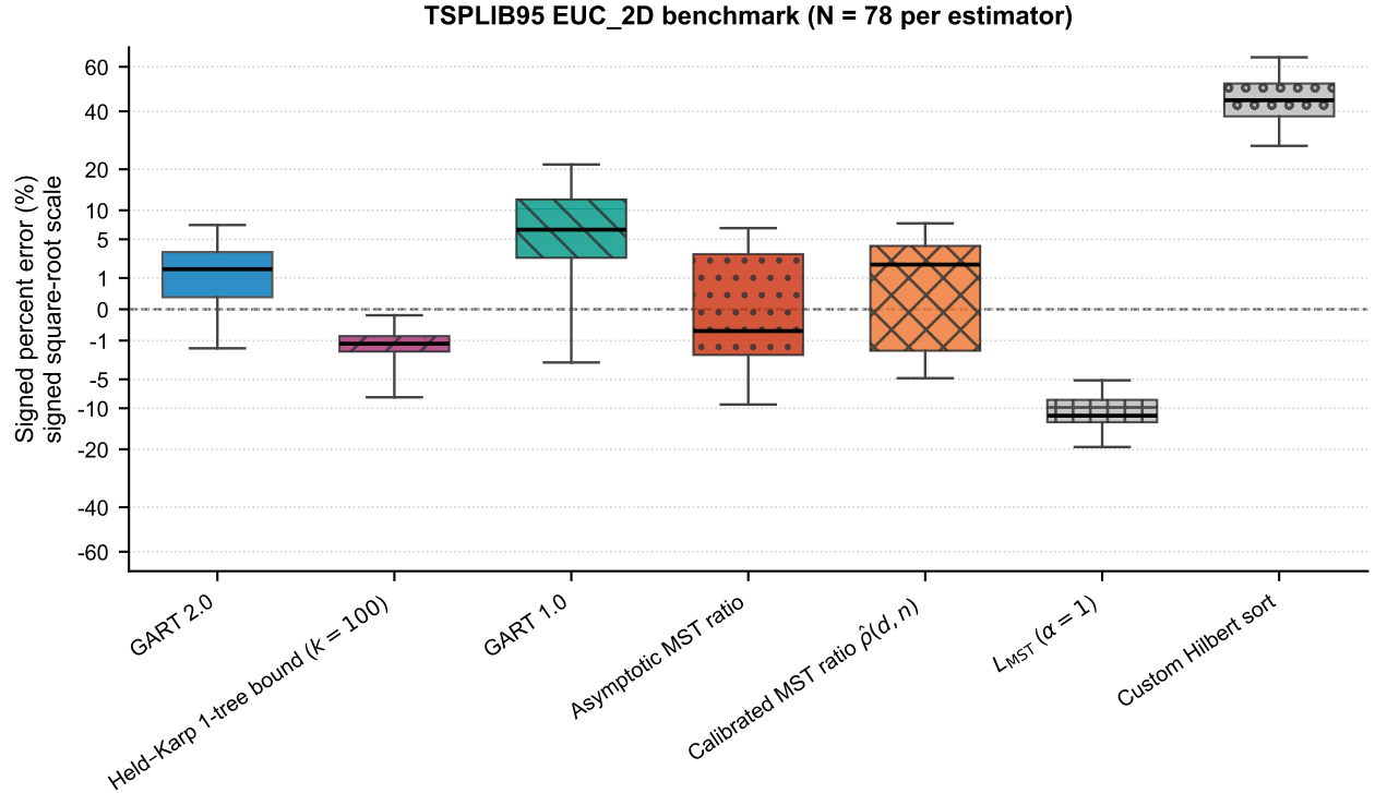
Figure 4: Signed percent error on the TSPLIB95 EUC_2D benchmark ( N = 78 per estimator). Boxes show the interquartile range and median; whiskers span the 5th–95th percentiles, and outliers are suppressed for legibility. The roster is that of Table 23 plus the certified Held–Karp 1-tree bound of Section 5 at ascent budget k = 100 . This is the stratum on which GART 2.0 is closest to the bound, and the two interquartile ranges sit on opposite sides of the zero line, GART 2.0’s just above it and the bound’s just below: the two err in opposite directions, and only one of them can be trusted not to overshoot. The vertical axis is the signed square root of Figure 1, on the same limits. The bound is scored here on all EUC_2D instances, including the one Table 3 excludes for cost, and on the released reference costs rather than the integer-rounded metric, which is why a few instances place it marginally above the reference.
