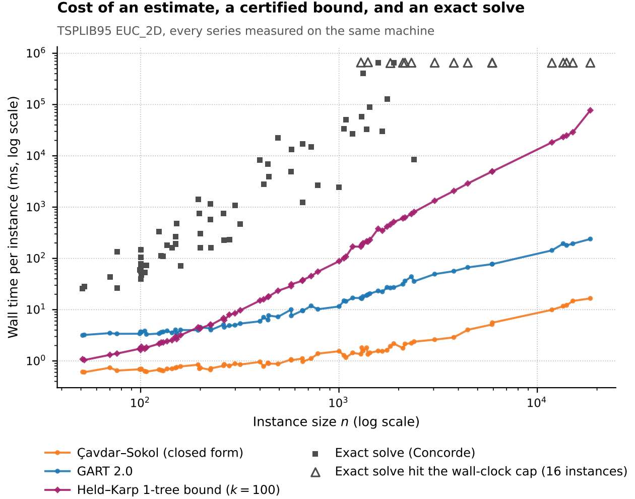
Figure 5: What each family costs per instance on TSPLIB95 EUC_2D, against instance size, both axes logarithmic. Every series is measured on the same machine, so the comparison needs no cross-hardware correction. The Çavdar-Sokol closed form is flat because it reads a handful of summary statistics; GART 2.0 rises gently because its planar extraction is subquadratic; the certified Held-Karp 1-tree bound, drawn at ascent budget k = 100 , rises steeply because each iteration costs \Theta(n^2) ; and the exact solve (Concorde) is scattered rather than joined because branch-and-cut time varies by orders of magnitude between instances of the same size. Open triangles are the runs that reached the wall-clock cap without proving optimality, so the exact curve is a lower bound on the solver’s true cost. The four families are separated by roughly five orders of magnitude at the largest instance.
