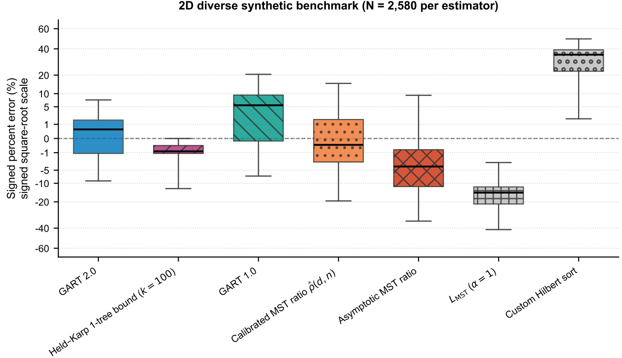
Figure 3: Signed percent error on the diverse 2D benchmark ( N = 2,580 per estimator). Boxes show the interquartile range and median; whiskers span the 5th–95th percentiles, and outliers are suppressed for legibility. The roster is that of Table 22 plus the certified Held–Karp 1-tree bound of Section 5, drawn at the same ascent budget k = 100 as in Figures 1 and 4; being one-sided it sits at or below zero. The vertical axis is the signed square root of Figure 1, on the same limits. The classical estimators are omitted from this figure only for legibility; their errors are an order of magnitude larger and are reported in Table 16.
