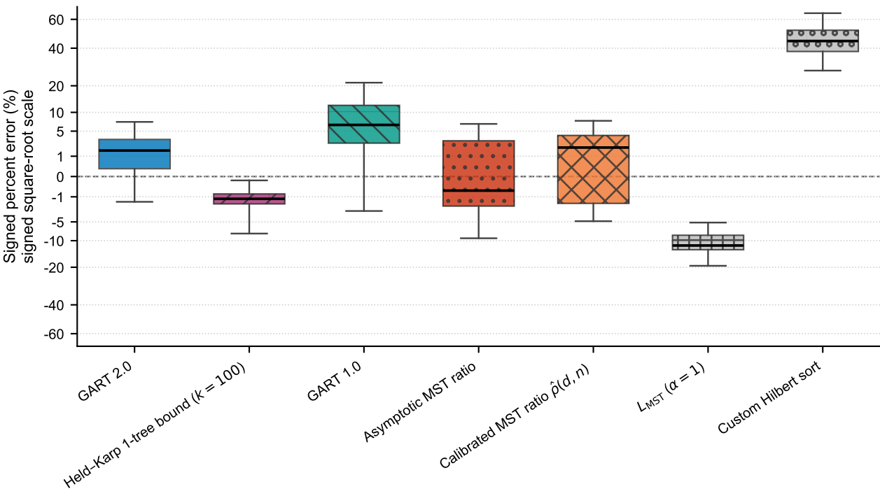
TSPLIB95 EUC_2D benchmark (N = 78 per estimator)
