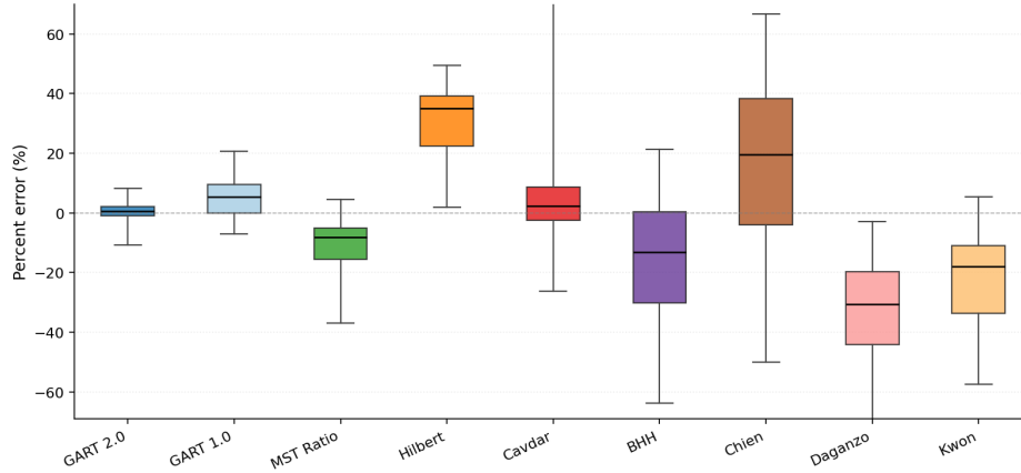
Figure 2: Percent-error distribution per model on the 2D diverse benchmark (2,580 instances).
