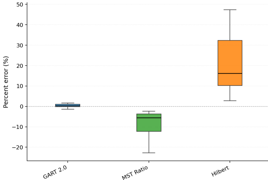
Figure 1: Percent-error distribution per model on the ND benchmark (16,920 instances).
