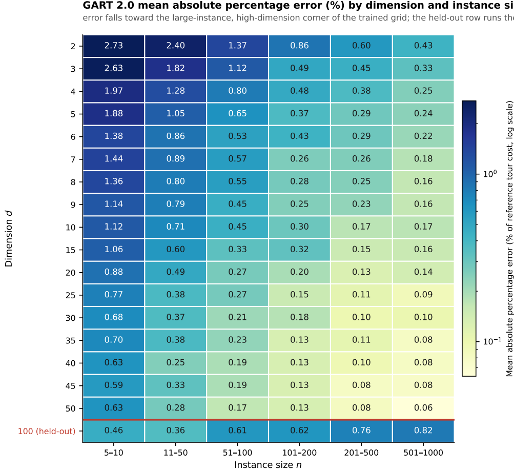
Figure 2: GART 2.0 MAPE by dimension and instance-size band; the red rule marks the held-out d = 100 row.
