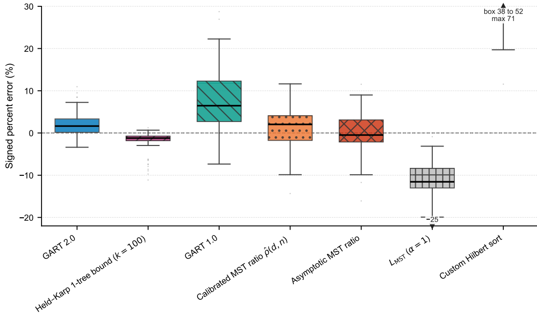
Figure 4: Signed percent error on the TSPLIB95 EUC_2D benchmark ( N = 78 per estimator).
