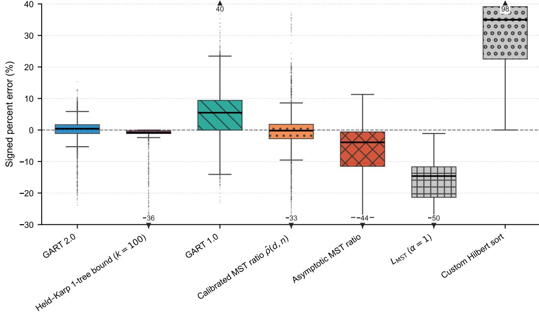
Figure 3: Signed percent error on the diverse 2D benchmark ( N = 2,580 per estimator).
