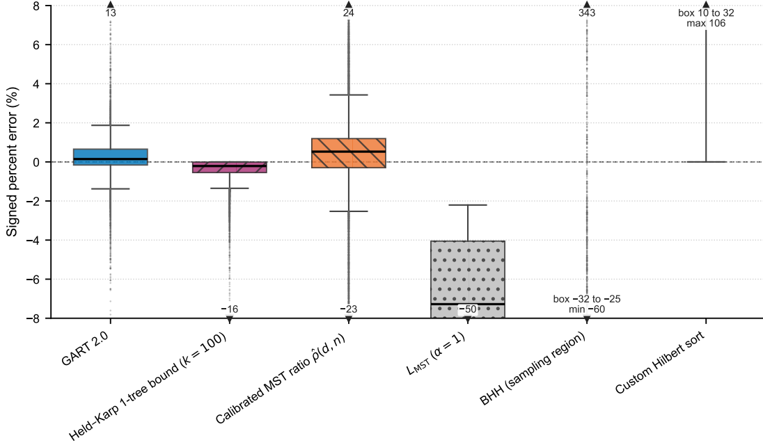
Figure 1: Signed percent error on the multidimensional benchmark ( N = 16,846 per estimator).
