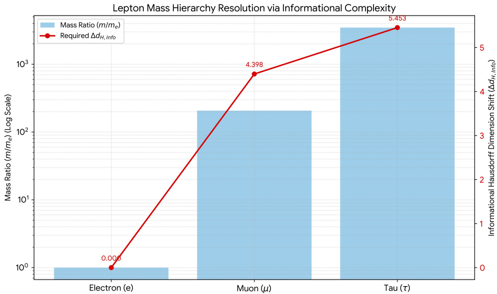
Figure 18.1: Lepton Mass Hierarchy Resolution. The exponential enhancement driven by the increase in Informational Hausdorff Dimension ( \Delta d_{H,\text{Info}} ) resolves the hierarchy. The required shifts ( \approx 4.4, 5.4 ) are plausible within the 24D Information Manifold.
