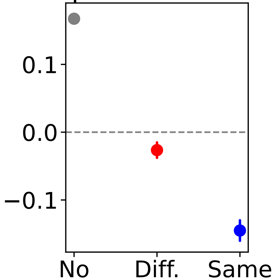
Sparse network
