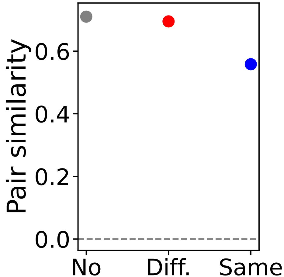
Dense network
