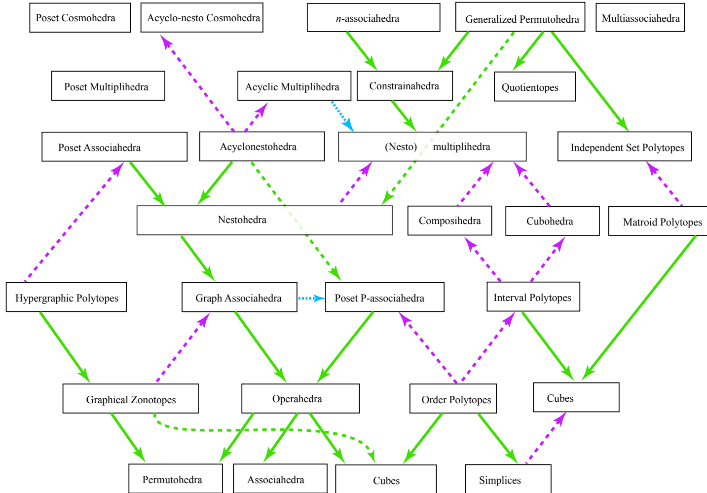
Figure 1: Some families of combinatorial polytopes. Solid green arrows point in the direction of subset containment: lower contained in upper. Dashed purple arrows show lifting, or collapse (in reverse). Dashed blue arrows indicate taking a cross section.
