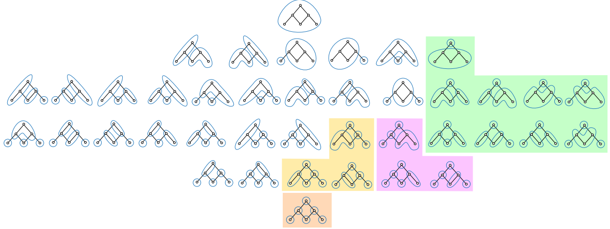
Figure 4: Faces of C_G \cong O(P'(G))^{\Delta} , for G the path graph with two edges. Highlighted on the right in four colors is the scattering facet F_G , a tetrahedron partitioned into the face posets of hypergraphic polytopes \Delta_G and its edge-deleted subgraph hypergraphic polytopes. The largest of these highlighted face posets is pictured as the hypergraphic polytope of the path graph in Figure 5.
