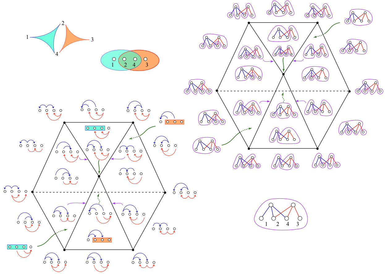
Figure 2: Example of the bijection in the proof of Theorem 5. The hypergraph G pictured two ways at far left has hyperedges E = \{\{1, 2, 4\}, \{2, 3, 4\}\} . The source sets of each hyperedge in the acyclic orientations are the starting nodes for each pair of same color arrows. When the source set is the entire hyperedge the nodes are highlighted. To the right is seen the corresponding labeling with acyclic connected partitions of P(G) , which is shown to be realized as a cross section of the polar dual of the order polytope.
