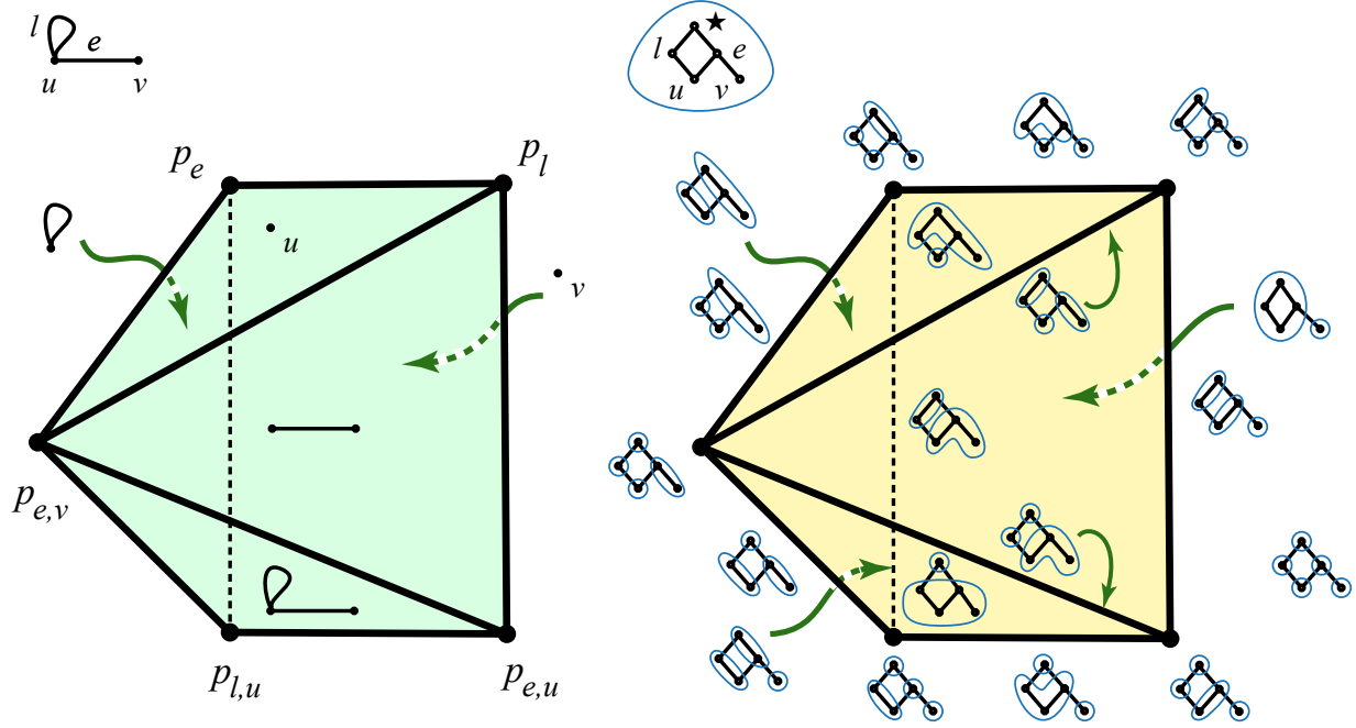
Figure 1: Left: the cosmological polytope C_G associated to the pseudograph G from Example 2. Right: the polar dual of the order polytope of the poset P'(G) , denoted O(P'(G))^\Delta ; the face lattice labeled by connected, acyclic partitions of P'(G) , as listed in Example 3 and demonstrating Theorem 3.
