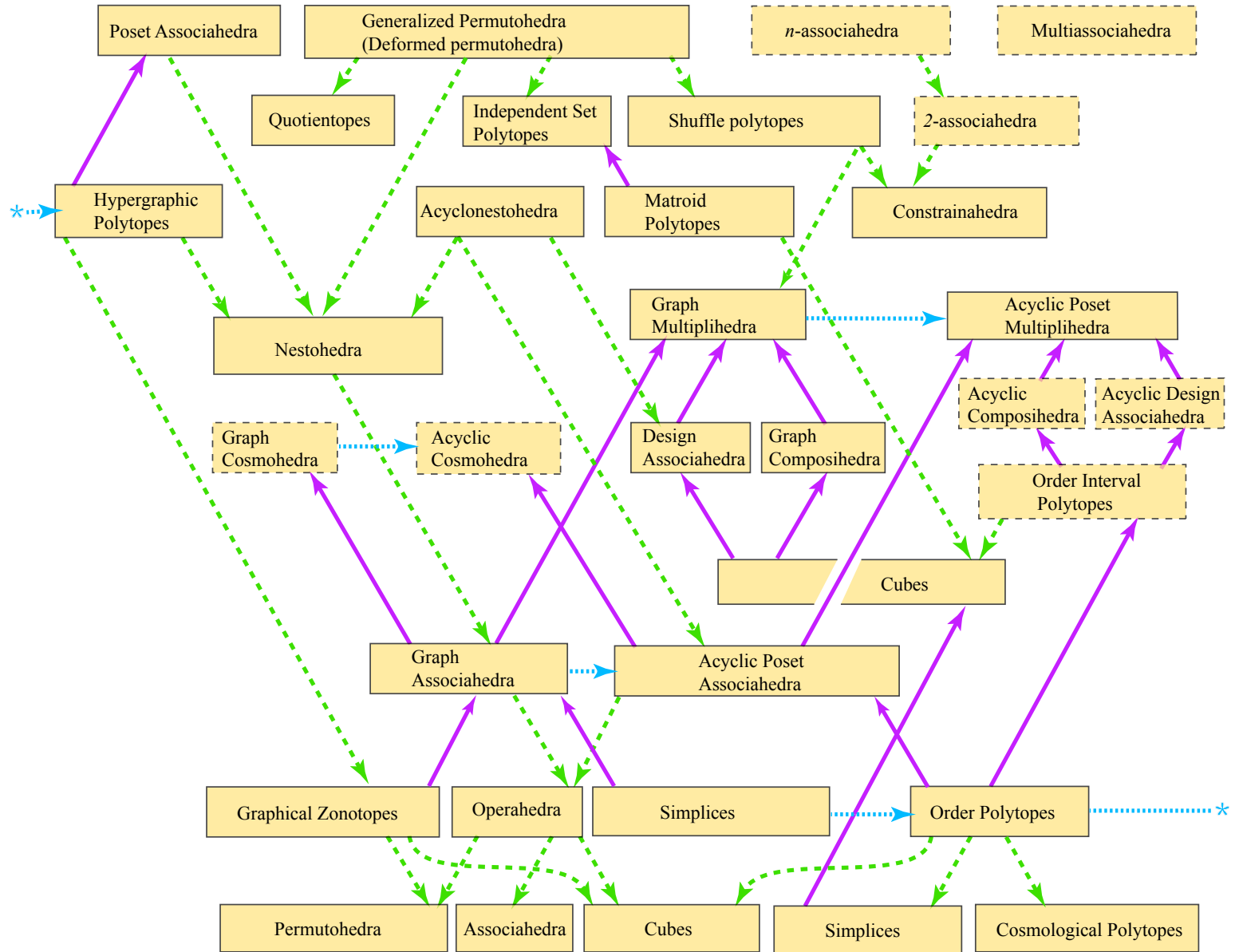
Figure 1: Relationships of families of polytopes: dashed green arrows slope down to indicate subset containment, lower contained in upper. Solid violet arrows point up to indicate lifting: refining the fan, truncation, taking intervals, or extending combinatorial structure. Dashed horizontal arrows show taking a cross section, left to right. Dashed boxes are conjectural polytopes.
