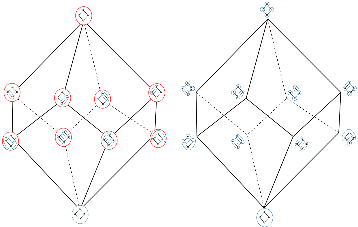
Figure 19: Vertex labels of the quotient of the diamond poset acyclic multiplihedron, under both equivalences: seen in bijection with the vertex labels of the interval polytope of the order polytope of the same poset. These vertices are the faces of the order polytope, as seen in Figure 4.
